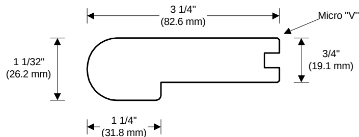
NOSING (SOLID FLOOR) NEZ DE PALIER (PLANCHER MASSIF)
