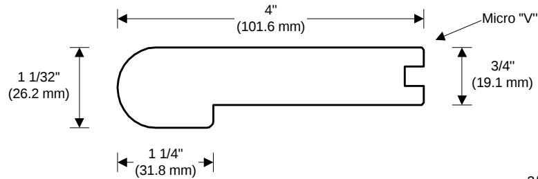
NOSING (SOLID FLOOR) NEZ DE PALIER (PLANCHER MASSIF)
