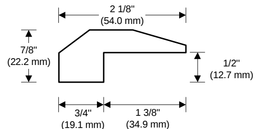
THRESHOLD (SOLID + ENGINEERED FLOOR) SEUIL (PLANCHER MASSIF + LAMINÉ)
